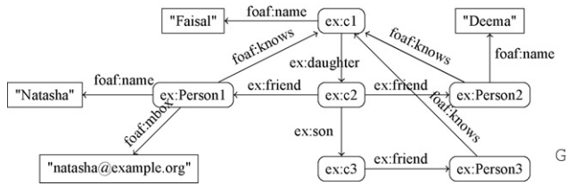
Fig. 1. An RDF graph.
