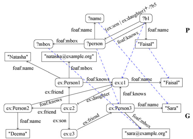
Fig. 5. A PRDF homomorphism from a PRDF graph to a GRDF graph represented in dashed lines.
