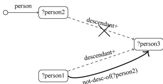
Fig. 9. A Graphlog query.
