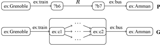
Fig. 6. A case in which the path closure method is not efficient.
