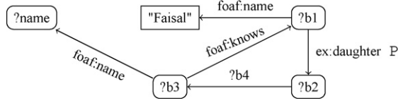
Fig. 3. A GRDF graph.
