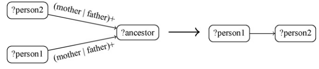
Fig. 8. A G+ query to find common ancestor.
