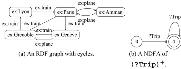
Fig. 7. An RDF graph and a NDFA. (a) An RDF graph with cycles. (b) A NDFA of (?Trip)^+ .
