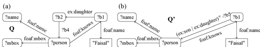
Fig. 2. A SPARQL graph pattern (a) and a PPARQL graph pattern (b).
