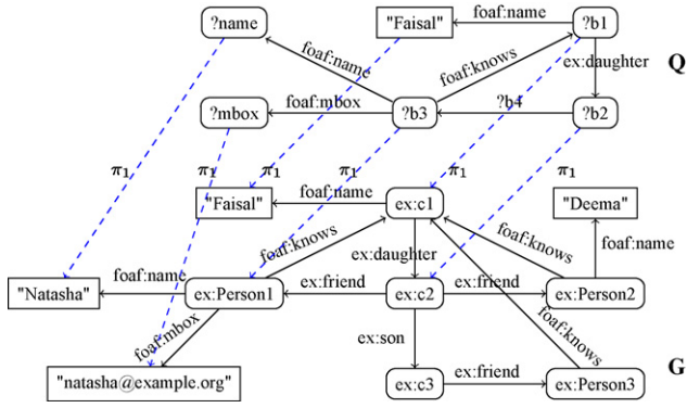
Fig. 4. An RDF homomorphism \pi from Q into G .
