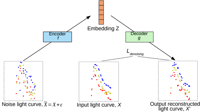
Fig. 4: Schema of the denoising autoencoder process.
