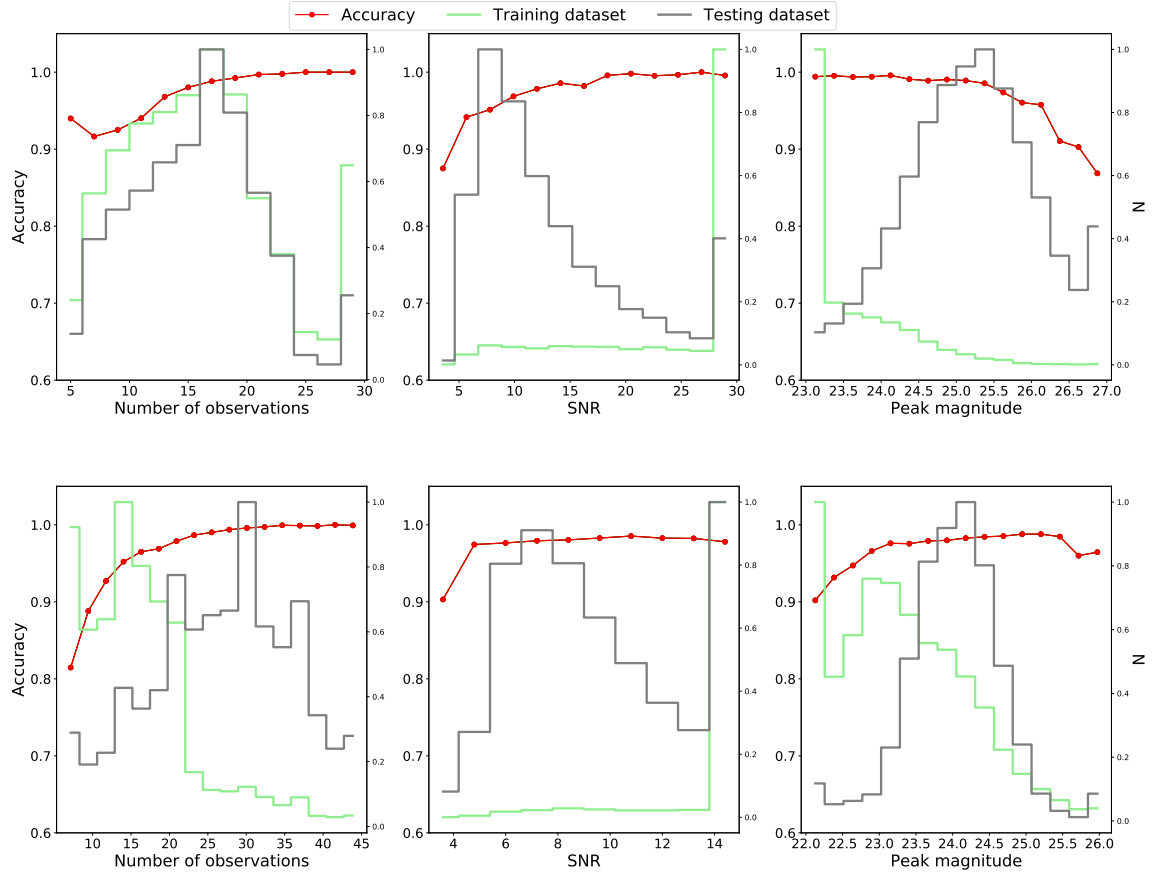
Fig. 12: The upper panels corresponds to the classification of DDF light curves and the lower panels to the classification of WFD light curves. Left panels : Accuracy as a function of the total number of observations on different dates for all bands. Middle panels : Accuracy as a function of SNR, which is computed as the maximum SNR from all bands. Right panels : Accuracy as a function of peak magnitude, which corresponds to the maximum value of peak magnitude from all bands. For each case the distribution of the training database is represented in light green and that of the test database in grey.
