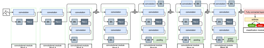
Figure 1.11 SRNet network.
