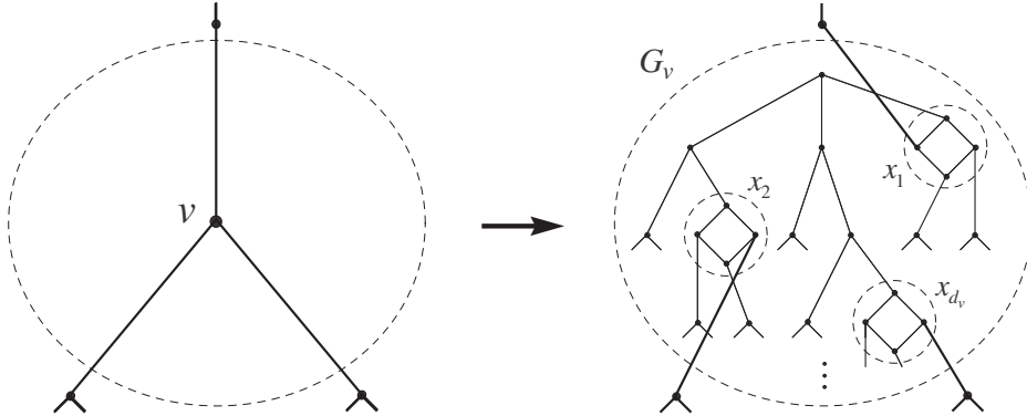
Fig. 2. Example of a graph G^2 \in \mathcal{G}_3^2 built in Section 2.1.
