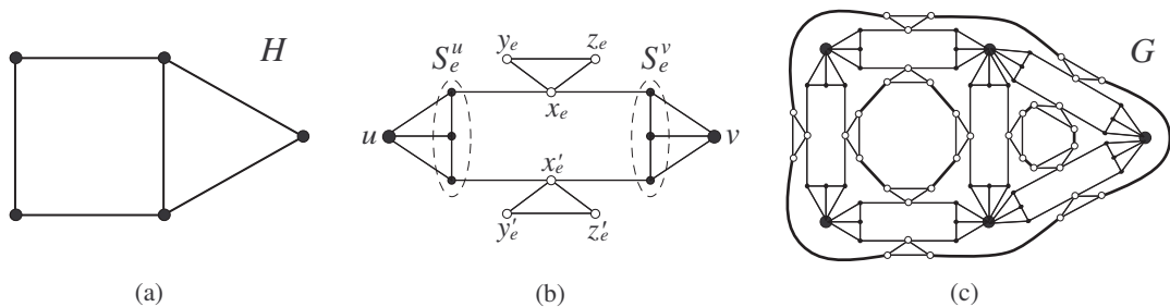
Fig. 3. Reduction in the proof of Theorem 5 for d = 3 : (a) Instance H of MINIMUM VERTEX COVER. (b) Gadget corresponding to an edge e = \{u, v\} \in E(H) . (c) Instance G of the 3-GIRTH problem built from H .
