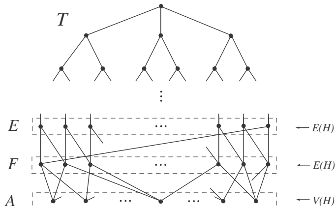
Fig. 1. Example of a graph G \in \mathcal{G}_3 built in Section 2.1.
