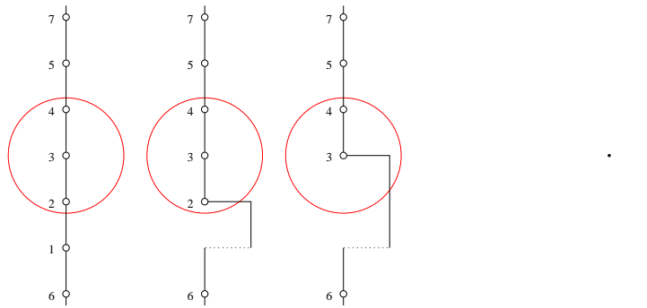
FIGURE 6. We take the same stepped surfaces \mathcal{S} and \mathcal{S}' as on Fig. 5. We consider the open ball B(\vec{0}, 1.25) (depicted as a circle). Following the proof of Prop. 2.5, we can sort the flips (as depicted on the figure) so that the projection \pi is a homeomorphism from the restrictions to B(\vec{0}, 1.25) of intermediate stepped functions onto their images under \pi .
