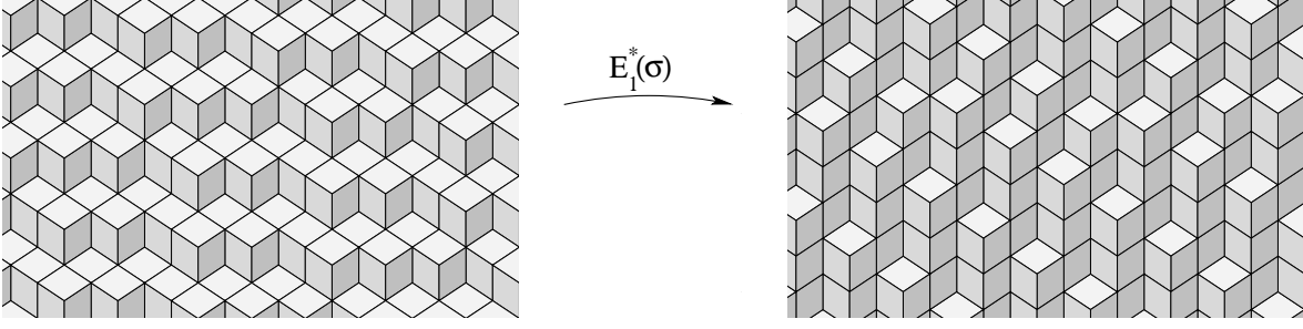
FIGURE 9. If the image of a stepped plane \mathcal{P}_{\vec{\alpha}, \rho} under a dual map E_1^*(\sigma) is a binary stepped function, then it is the stepped plane \mathcal{P}_{M_\sigma^{-1}\vec{\alpha}, \rho} .
