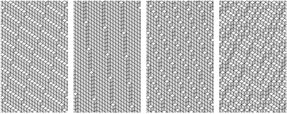
FIGURE 14. Iterated applications of the map \tilde{T} on a stepped surface (from left to right). Note that stepped surfaces are more and more bumpy, due to the contracting effect of \tilde{T} .
