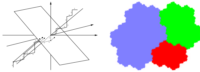
Figure 7: The projection method to get the Rauzy fractal for the Tribonacci substitution.
