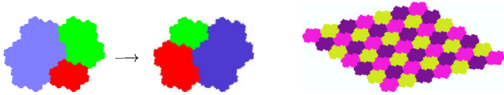
Figure 8: Domain exchange over the Rauzy fractal; lattice substitution multiple tiling
