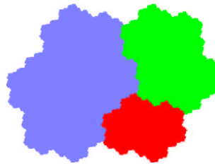
Figure 1: Tribonacci substitution: the central tile divided into its basic tiles.
