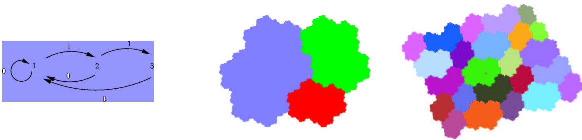
Figure 4: Tribonacci number: the minimal automaton \mathcal{M}_\beta , the central tile divided into its basic tiles; the self-replicating multiple tiling.
