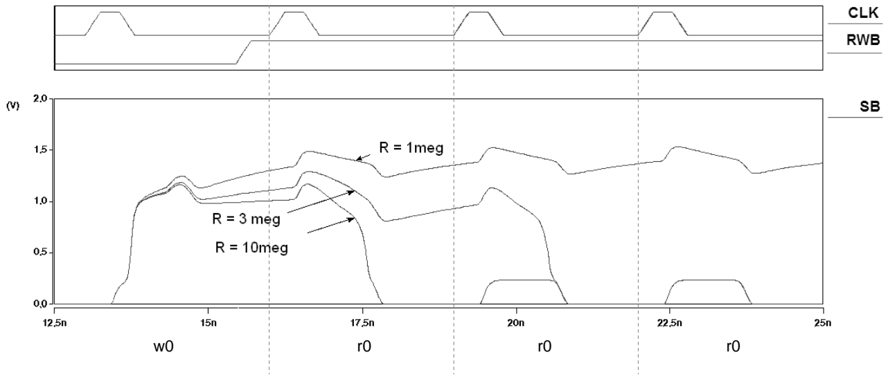
Figure 5: A destructive read occurring after consecutives “at-speed” read access (typ proc, T=125°C, V=1.6V, T cyc =3ns)
