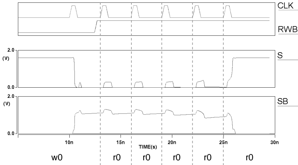
Figure 6: A destructive read occurring after the 5 th consecutive “at-speed” read access (typ proc, T=125°C, V=1.6V, T cyc =3ns, R=1.5MΩ)
