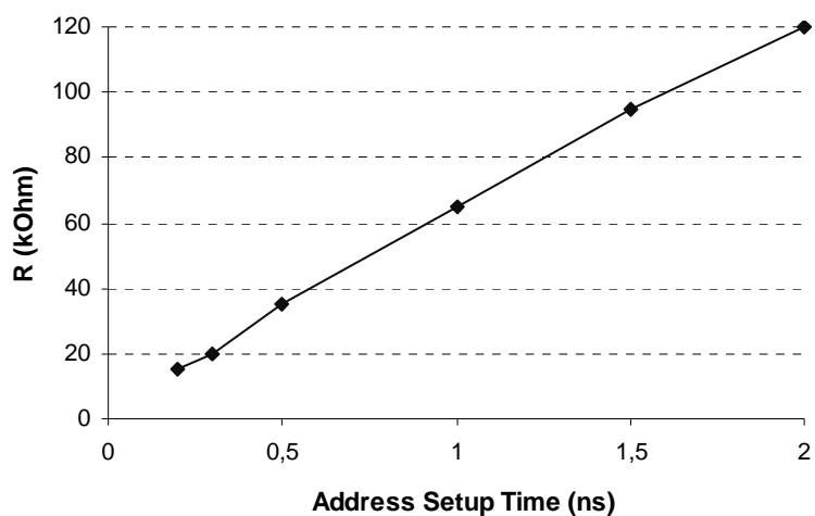
Figure 9: Minimum detected resistance vs. address setup time (typ proc, T=27°C, V=1.5V)
