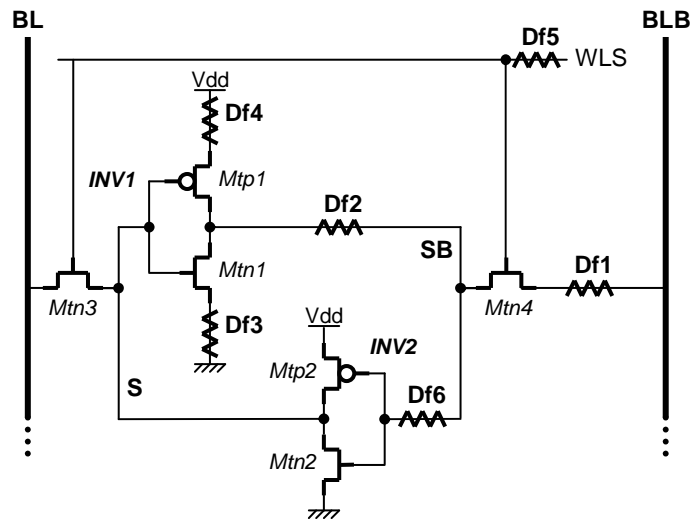
Figure 1: Resistive-open defects injected in the memory core-cell
