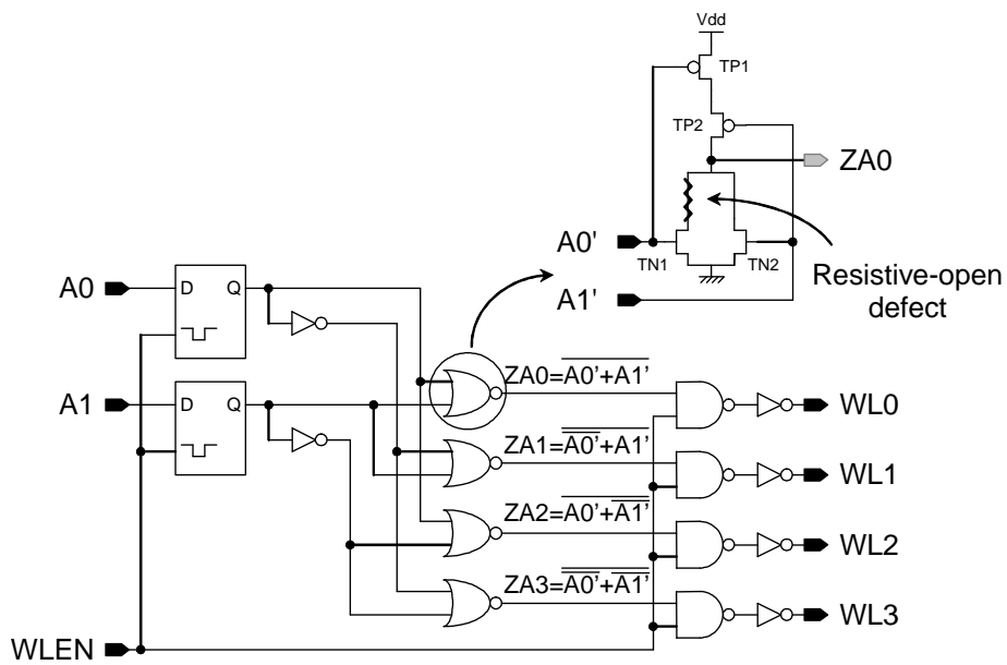
Figure 2: Intra-gate resistive-open in the pull-down path of NOR-based address pre-decoder
