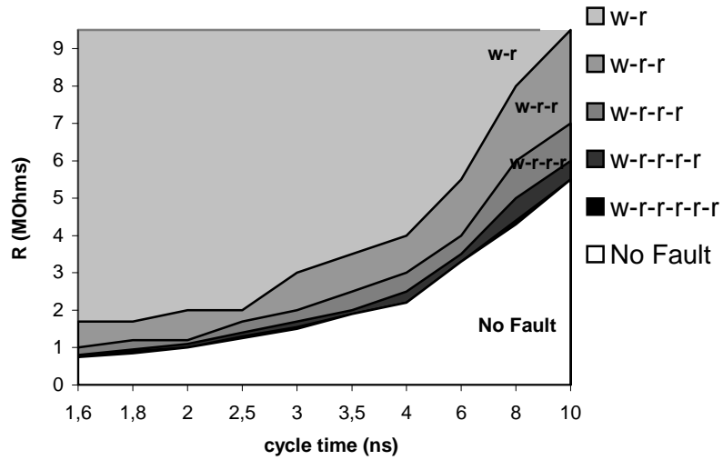
Figure 7: Defect detection as a function of cycle-time for different sensitization sequences (typ proc, T=125^{\circ}\text{C} , V=1.6\text{V} )
