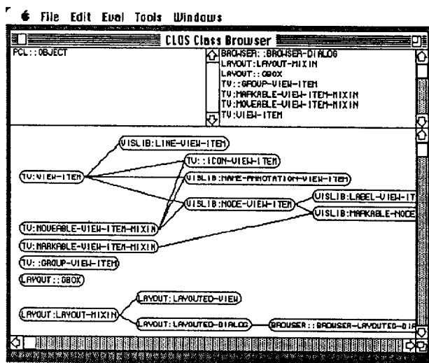
Figure 2: A DAG graph of a standard class hierarchy.
