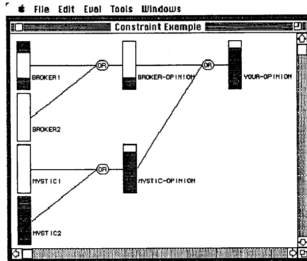
Figure 5: The upper and lower bounds are indicated by shaded rectangles [28]. The gauges show the estimation interval from 0 (bottom) to 1 (top).
