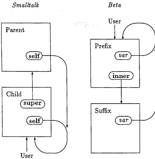
Figure 1: Inverse hierarchies in Smalltalk and Beta.
