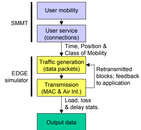
Figure 5: Relationship between the SMMT and the system simulator
