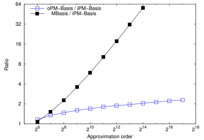
Figure 3: Relative performance of two online order basis algorithms against polynomial matrix multiplication. The input matrix power series are in \mathbb{F}_p[x]^{32 \times 16} for p a 23-bit prime.
