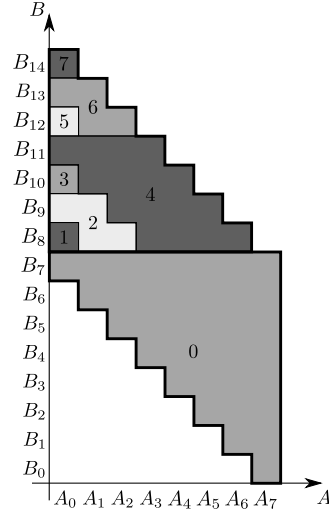
Figure 1: Shifted online middle product \text{MP}(A, B, 8)
