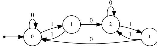
Fig. 1. 2-DFAO for \text{vtm}
