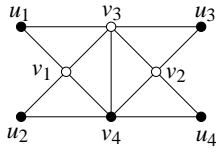
Fig. 6. Unavoidable configuration in a 2-outerplanar graph containing neither a \leq 3 -vertex, nor two adjacent 4-vertices
