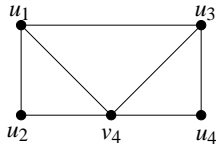
Fig. 7. Reduction of the configuration depicted in Figure 6
