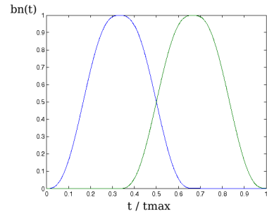
Fig. 1. Representation of B-splines functions b_n(t) with n_b = 2 .
