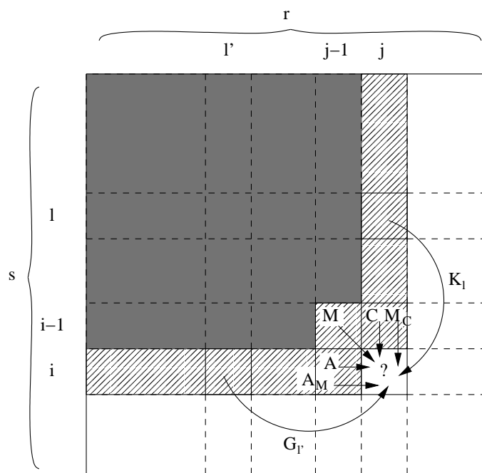
Fig. 10. Dependencies in the dynamic programming matrix. To compute cell A(i, j) , we need at most all cells in the striped patch but not the ones in the dark patch. Dependencies are shown by arrows. For arch generations and compression the arrows are indexed by the beginning position of the arch to show that there are multiple dependencies.
