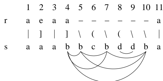
Fig. 9. Alignment of the maps r := aeaaa and s := aaabbcbddba . The arch bbcbddba and its inner-arches are drawn by curved lines under s . In the middle line, '|', ']', '\', '(' denote resp. a match, a mismatch, an amplification, and an amplification+mutation.
