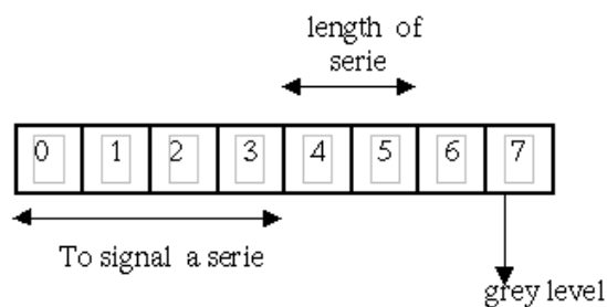
Figure 6. Crypto-compression method.
