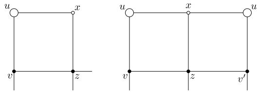
Fig. 5. Some configurations that appear in Lemma 12.
