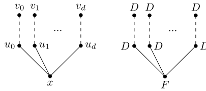
Fig. 8. The gadget H in Case 1, and an (\mathcal{F}, \mathcal{F}_d) -partition. Dashed lines are anti-edges.
