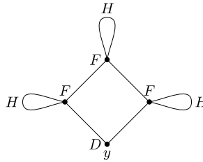
Fig. 10. The gadget H' with an (\mathcal{F}, \mathcal{F}_d) -partition.
