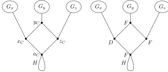
Fig. 11. The cycle K_C of a clause C with variables x, y and z , and an (\mathcal{F}, \mathcal{F}_d) -partition in the case where variable x satisfies the clause.
