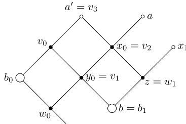
Fig. 7. The case in Lemma 13 where y_0 corresponds to v_1 in Configuration 1.
