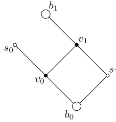
Fig. 1. The forbidden configuration of Lemma 8. The big vertices are represented with big circles, and the small vertices with small circles. The filled circles represent vertices whose incident edges are all represented.
