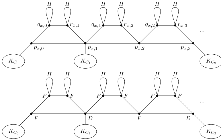
Fig. 12. The gadget G_x for a variable x , with an (\mathcal{F}, \mathcal{F}_d) -partition that corresponds to the assignment of x to true. Here the literal associated to x in C_0 is positive, and that associated to x in C_1 and C_2 is negative.
