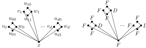
Fig. 9. The gadget H in Case 2, and an (\mathcal{F}, \mathcal{F}_d) -partition.
