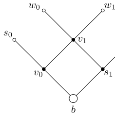
Fig. 2. The forbidden configuration of Lemma 9.
