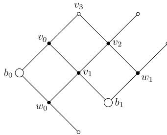
Fig. 4. The forbidden configuration of Lemma 10.
