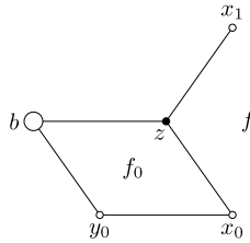
Fig. 6. The face f_0 and the vertex x_1 .
