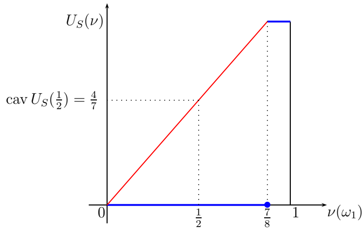
Figure 2: Concavification.
