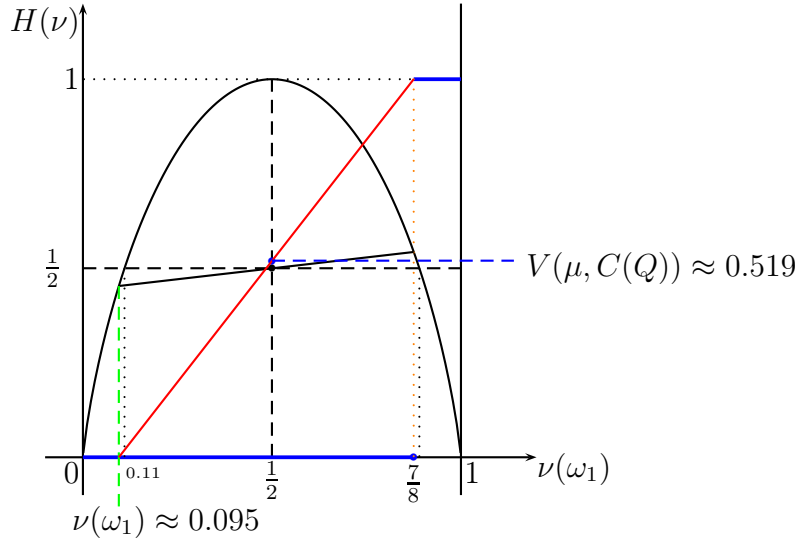
Figure 7: Optimal splitting with small perfect channel
