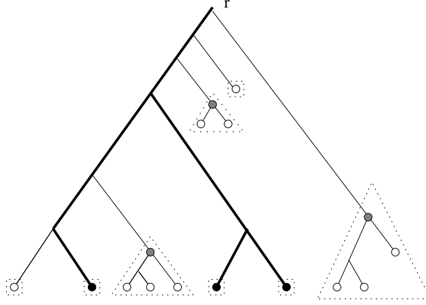
Figure 2: Illustration of the construction of \mathcal{P} . The black vertices belong to G \setminus D_2 and the bold edges represent S . The partition \mathcal{P} is pictured by the dotted sets, while its associated nodes u are in grey.
