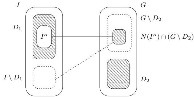
Figure 1: Illustration of the case |I''| > |N(I'') \cap (G \setminus D_2)| . The dashed sets represent the vertex cover D' .
