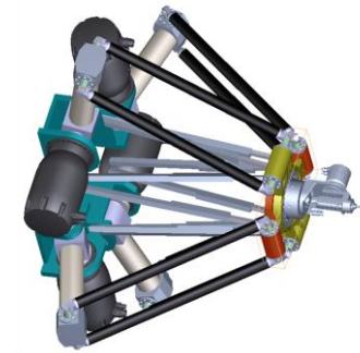
Image: SPIDER4 PKM ©: LIRMM
