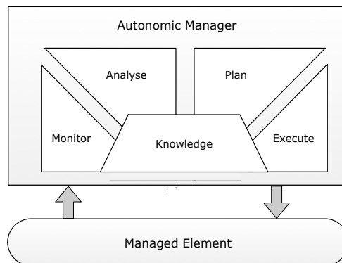
Figure 3: Structure of autonomic manager (based on [36])
