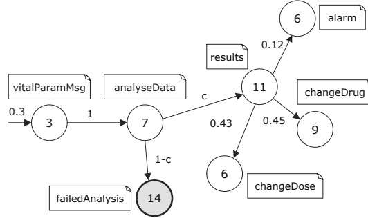
Figure 12: Excerpt of DTMC model for Tele-assistance system (based on [13])
