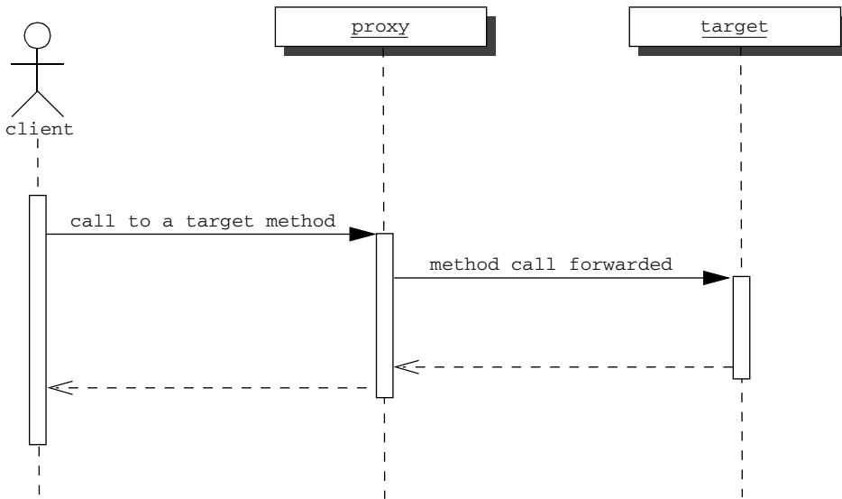
Figure 4.1 Sequence diagram for the typical use of a proxy. The proxy forwards received method calls to its target. The proxy may or may not do some pre- and post-processing.
