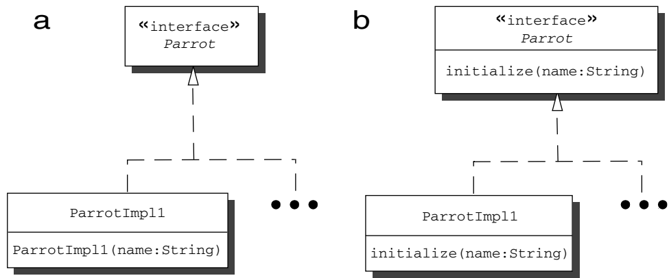
Figure 3.3 a) The left side shows implementations of Parrot using constructors with arguments to initialize themselves. b) The right side shows Parrot implementations using a method introduced by Parrot to initialize themselves.
