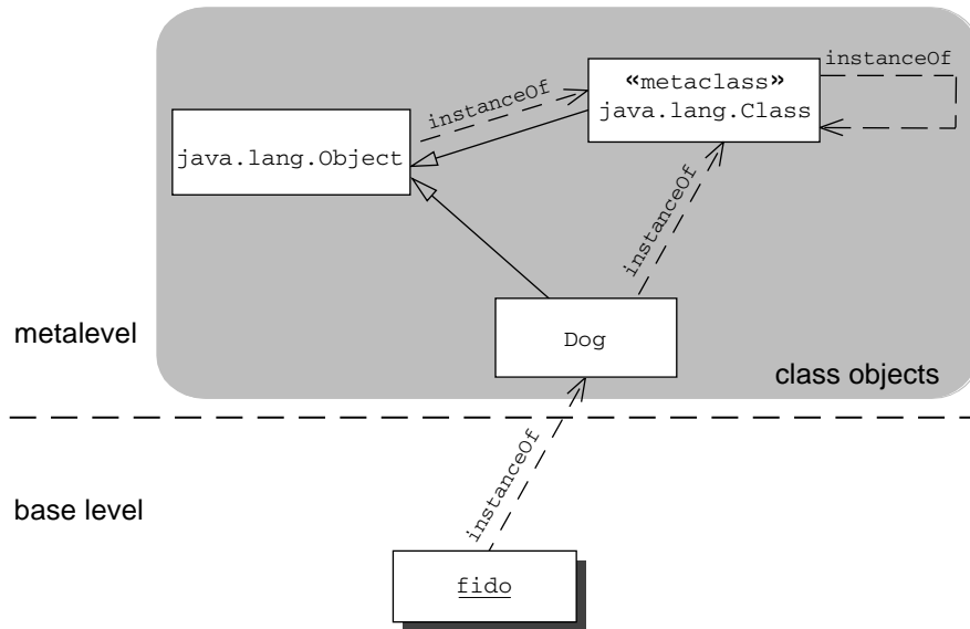
Figure 1.6 Object is the top of the Java inheritance hierarchy, so classes of metaobjects, including Class, are subclasses of Object. This means that the methods of Object are part of the reflection API. All Java classes are instances of its only metaclass, Class. These two conditions create a cycle in the diagram.
