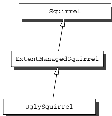
Figure 7.3 The instances of UglySquirrel are included in the extent of ExtentManagedSquirrel because constructors of ExtentManagedSquirrel must participate in creating instances of UglySquirrel .
