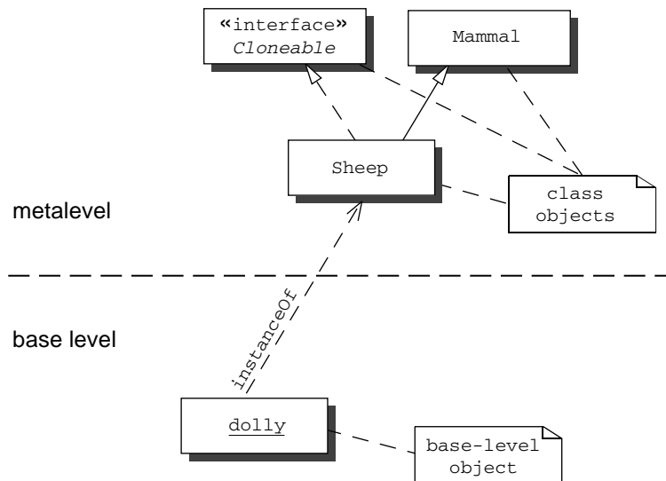
Figure 1.4 This is a Unified Modeling Language (UML) diagram describing Dolly the cloned sheep. The diagram shows an object, dolly , which is an instance of the class Sheep . It describes Sheep as a Mammal that implements Cloneable . The important thing to notice about this diagram is that it includes both objects and classes, as is necessary for describing reflective systems.
