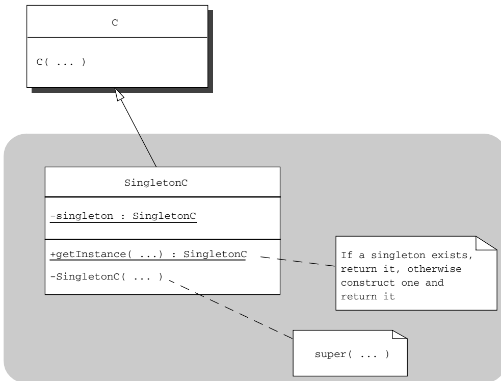
Figure 8.1 Design for the outcome of applying the Singleton pattern on the class C with the use of the C2SingletonC transformation. The resulting class SingletonC makes the constructor private while providing a factory method and a new private instance variable to hold the location of the singleton.
