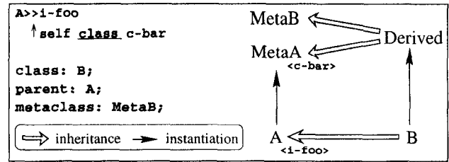
Figure 5: SOM ensures upward compatibility using derived metaclasses
