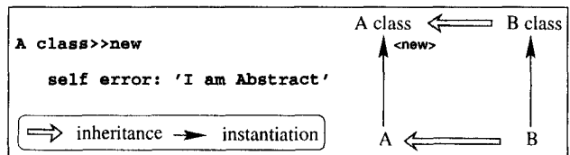
Figure 9: Class property propagation in SMALLTALK
