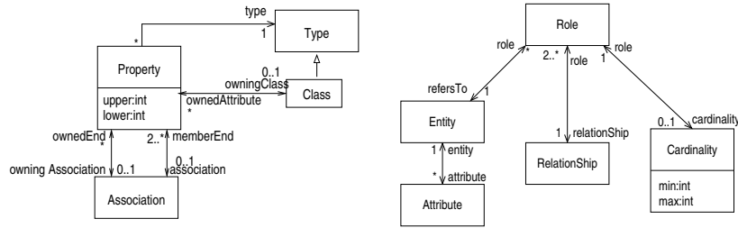
Fig. 1. Simplified metamodel for UML (lhs) and Entity-Relationship (rhs) used in [7].
