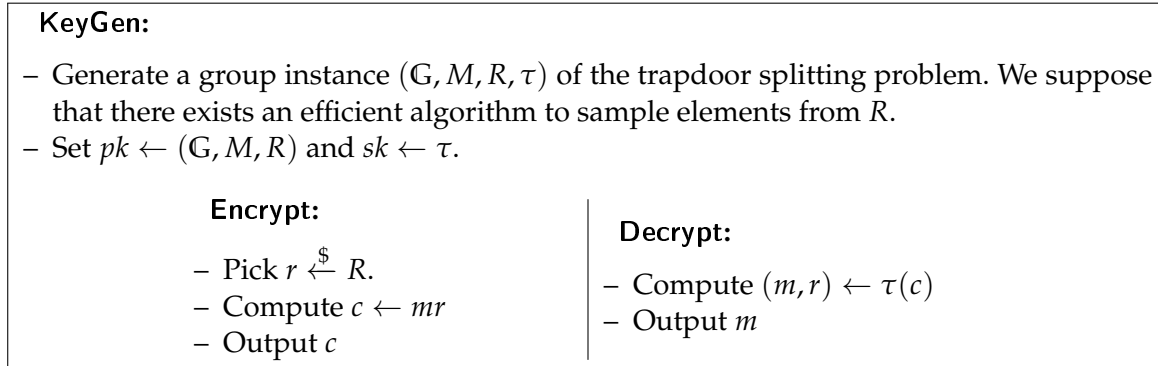
Figure 1.4 – General framework for homomorphic encryption
