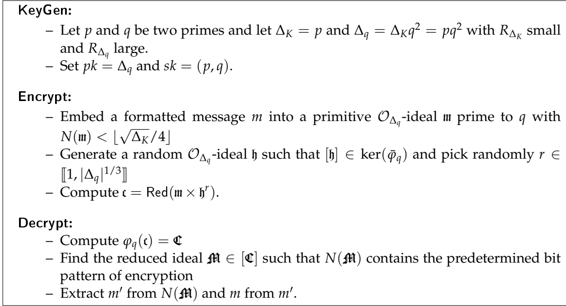
Figure 1.7 – Description of NICE in real quadratic fields
