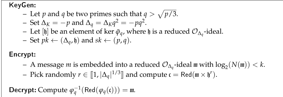
Figure 1.5 – Simplified Description of the original NICE
