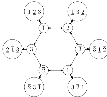
Fig. 1. The graph of adjacencies between the symbols of \bar{\mathbb{A}} and \bar{\kappa} -triples, and the mappings defined by \kappa .
