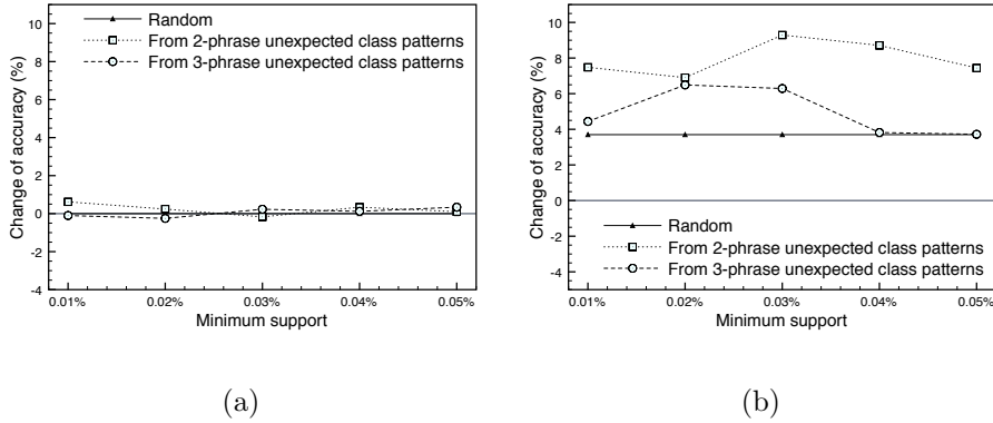
Figure 8: Change of average accuracy before and after eliminating unexpected sentences by using TFIDF method: (a) without pruning the most frequent common words; (b) with top-10 the most frequent common words pruned.
