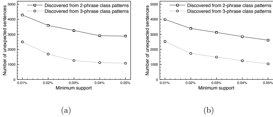
Figure 4: Number of unexpected sentences discovered from 2-phrase and 3-phrase unexpected class patterns of: (a) the class “positive”; (b) the class “negative”.
