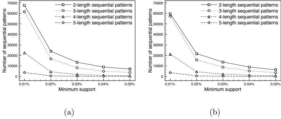
Figure 1: Number of discovered sequential patterns with different sequence length of: (a) the class “positive”; (b) the class “negative”.
