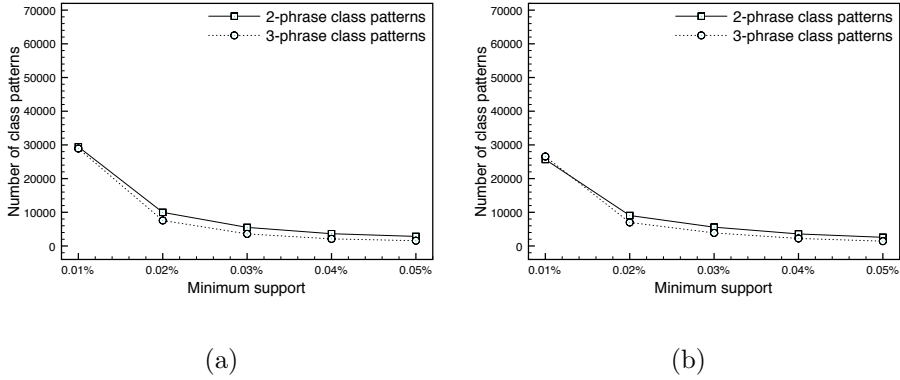
Figure 2: Number of 2-phrase and 3-phrase class patterns of: (a) the class “positive”; (b) the class “negative”.
