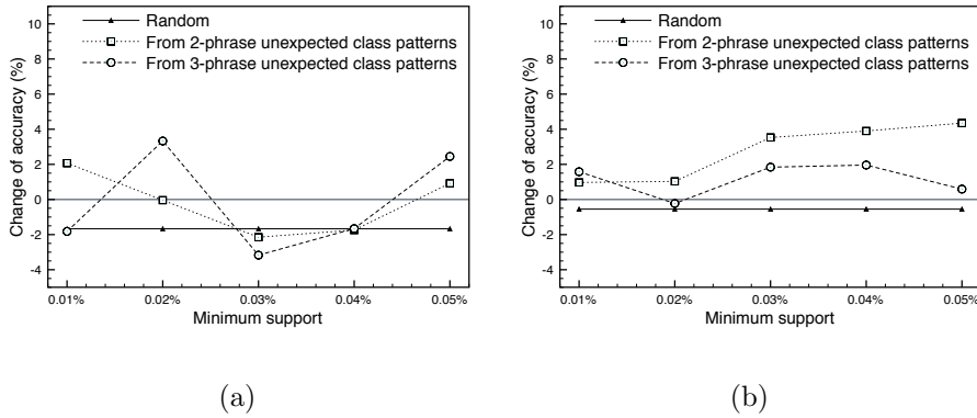
Figure 6: Change of average accuracy before and after eliminating unexpected sentences by using k -NN method: (a) without pruning the most frequent common words; (b) with top-10 the most frequent common words pruned.
