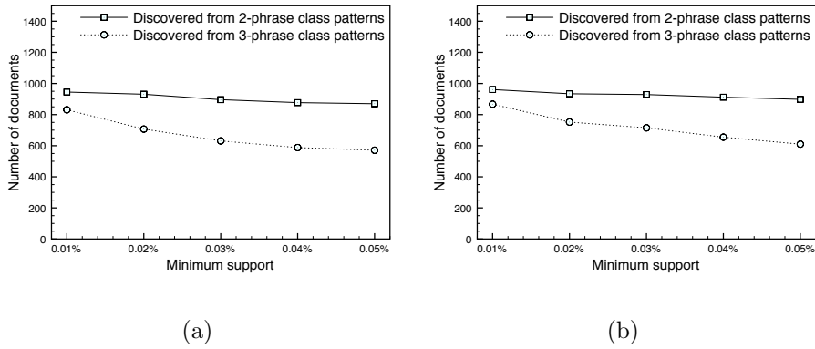
Figure 5: Number of documents that contain unexpected sentences discovered from 2-phrase and 3-phrase unexpected class patterns of: (a) the class “positive”; (b) the class “negative”.
