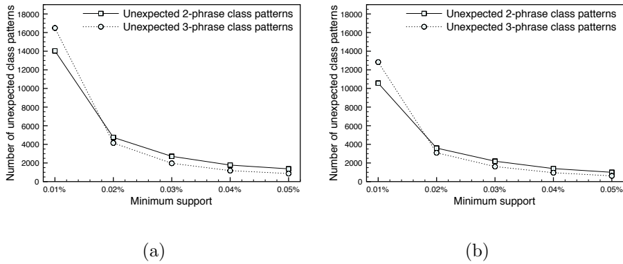
Figure 3: Number of 2-phrase and 3-phrase unexpected class patterns of: (a) the class “positive”; (b) the class “negative”.
