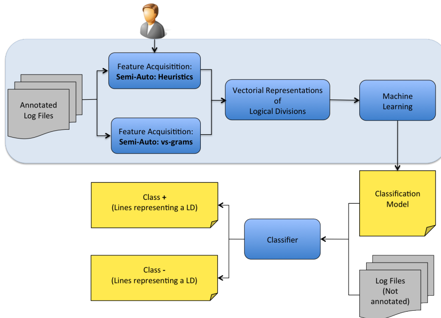
Figure 3: The global process of logical structure recognition.
