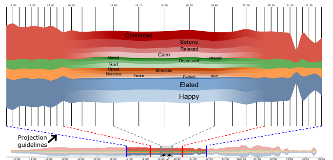
Fig. 7. At the bottom, the controller shows the areas displayed in the multiresolution view. At the top, the multiresolution view, result of the controller projection. Colored projection guidelines help the viewer to follow these projections.
