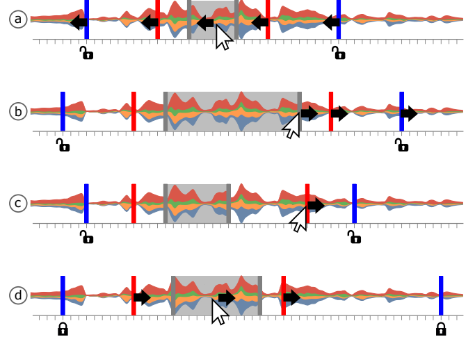
Fig. 6. Using the controller. (a) Detailed-area is dragged to the left. (b) Detailed-area is expanded to the right. (c) Right transition-area is expanded to the right. (d) The position of the context-areas are locked by clicking the padlock icon.
