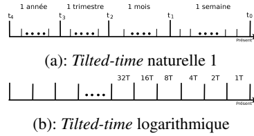
Figure 3 – Exemples de tilted-time
