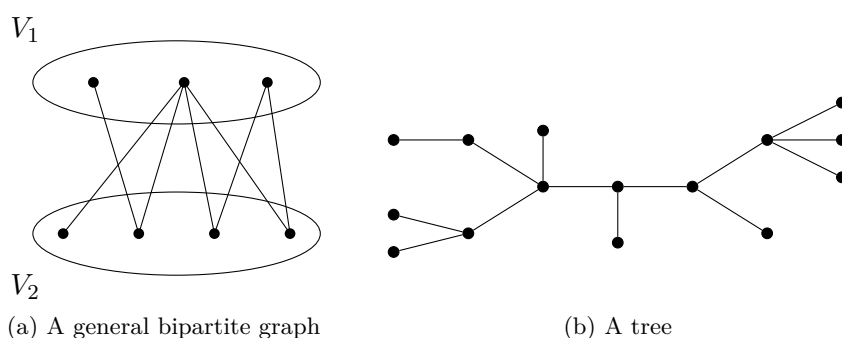
Figure 1.1: Bipartite graphs
