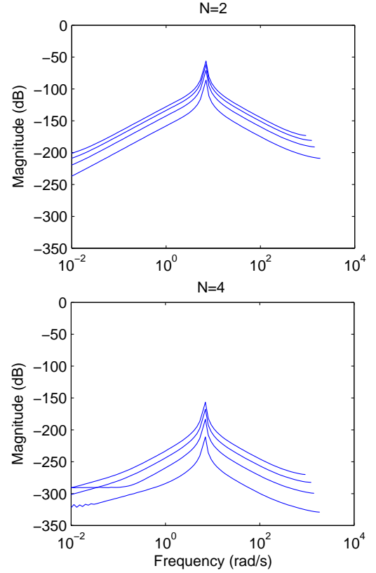
Fig. 9. |G_{d_e}(\delta_h, z) - G_d(\delta_h, z)| for \neq h - Taylor order 2 and 4
