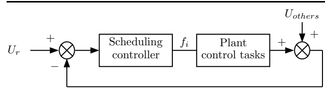
Figure 2. Feedback scheduling bloc diagram
