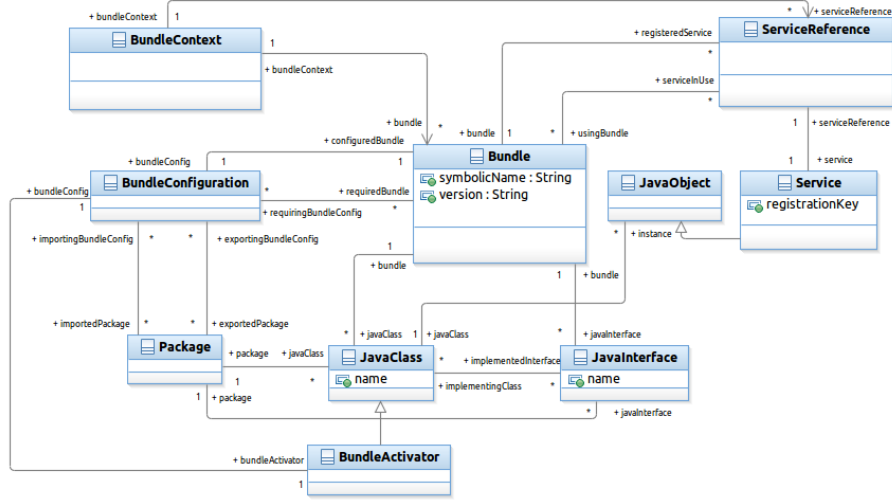
Figure 6: OSGi metamodel
