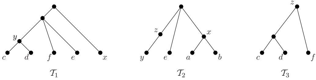
Figure 1: A compatible collection \mathcal{P} of rooted semi-labelled trees.
