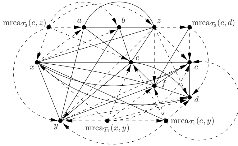
Figure 4: The descendanty graph of \mathcal{P}' . Arcs are shown as dashed lines with an arrow showing the direction of the arc, while edges are shown as solid lines.
