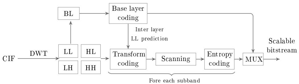
Fig. 8. DWTSB scalable architecture based on H.264/AVC.
