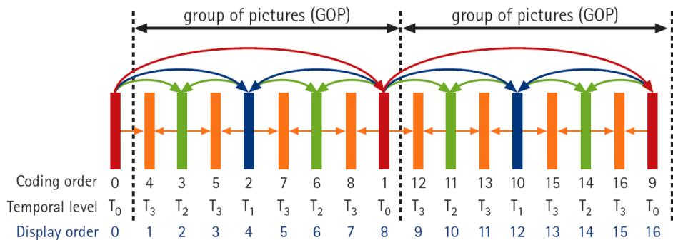
Fig. 4. Temporal scalable architecture of Scalable extension of H.264/AVC.
